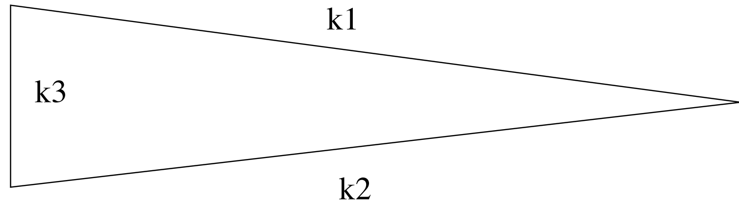
(a) Squeezed
