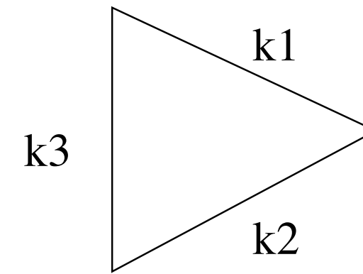
(b) Equilateral
