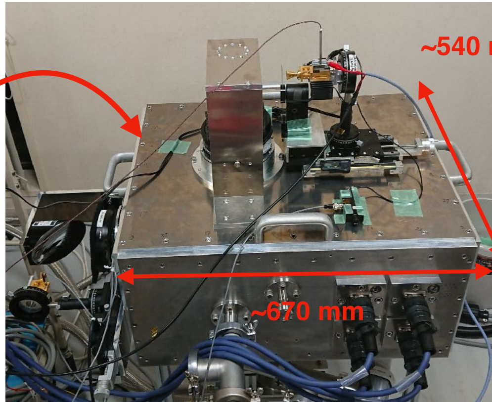
Rotation mechanism
