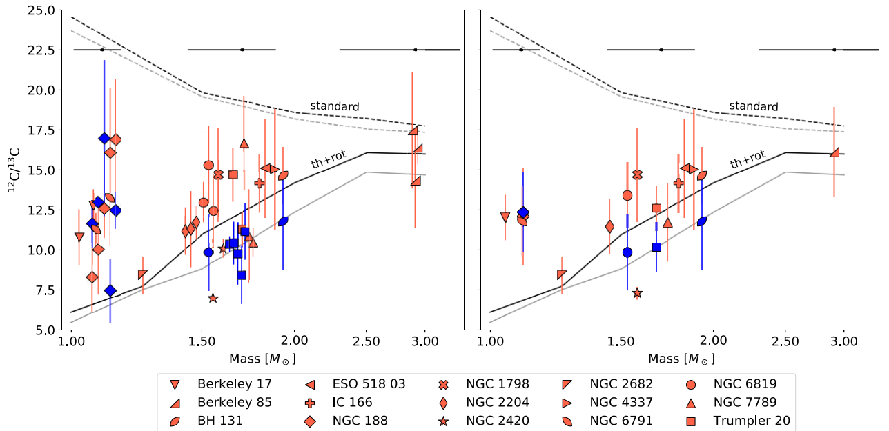
Figure 6. The same as Fig. 5, but as a function of the initial stellar mass for stars at the cluster main sequence turn off instead of stellar age. Horizontal, black error bars at the top of each figure represent typical mass errors.
