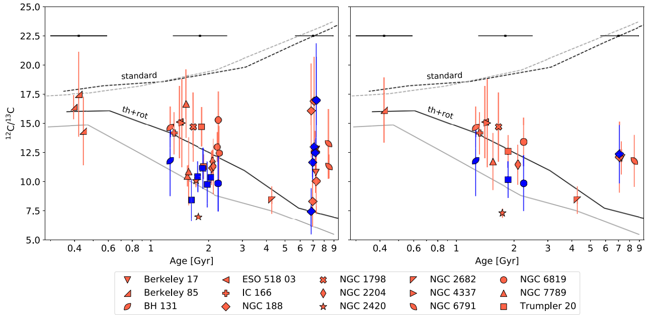
Figure 5. The ^{12}\text{C}/^{13}\text{C} ratio as a function of age for individual open cluster stars ( left ) and mean cluster values ( right ). Blue data points correspond to red clump stars undergoing core He-burning, and orange data points correspond to stars on the RGB. Individual stars in a given cluster, or at the same age, are intentionally offset slightly in age to better show the ^{12}\text{C}/^{13}\text{C} error bars. Horizontal, black error bars at the top of each figure represent typical age errors. Overlaid are curves showing the ^{12}\text{C}/^{13}\text{C} and age values at the tip of the RGB from the Lagarde models assuming: (1) standard stellar evolution ( dashed curves ), and (2) thermohaline mixing and stellar rotation ( solid curves ), for [\text{Fe}/\text{H}] = 0 ( black ) and [\text{Fe}/\text{H}] = -0.56 ( grey ).
