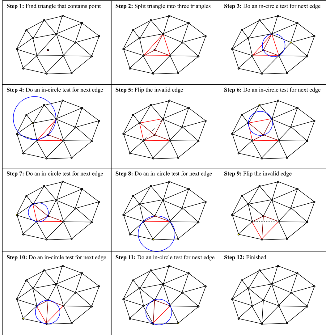
Figure 2. The point insertion algorithm in 2D. We start with a valid Delaunay triangulation in which we want to insert an additional point. We first locate the triangle containing the point (step 1), then split it into three triangles (step 2). The edges (drawn in red) in the new triangles opposite of the inserted point may violate the in-circle criterion and need to be tested individually. If an edge is Delaunay (step 3), it is part of the final tessellation, but if it violates the in-circle criterion (step 4), the edge needs to be flipped in the quadrilateral formed by the adjacent triangles (step 5). The flip generates additional edges that need to be tested (steps 6 and 7). Any violating edge found (e.g. step 9) needs to be corrected by flips. Once all remaining new edges are validated (steps 10 and 11), we arrive again at a valid Delaunay tessellation (step 12).
