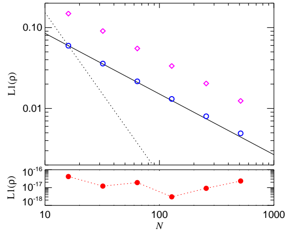
Figure 20. L1 error norm for a contact discontinuity (a density step from \rho = 1 to \rho = 2 that moves once through a box). The blue circles show the error as a function of resolution when we use our code with a Cartesian mesh with a fixed grid. In the presence of the discontinuity and the need to advect it the global rate of convergence is reduced to only about L1 \propto N^{-3/4} . However, for the moving-mesh code, shown with red circles, the error is consistent with zero within floating point rounding errors. For comparison, we also show with diamonds the L1 error of the same test carried out with ATHENA (using 2nd order reconstruction and the Roe solver). The dotted line illustrates a second-order scaling.
