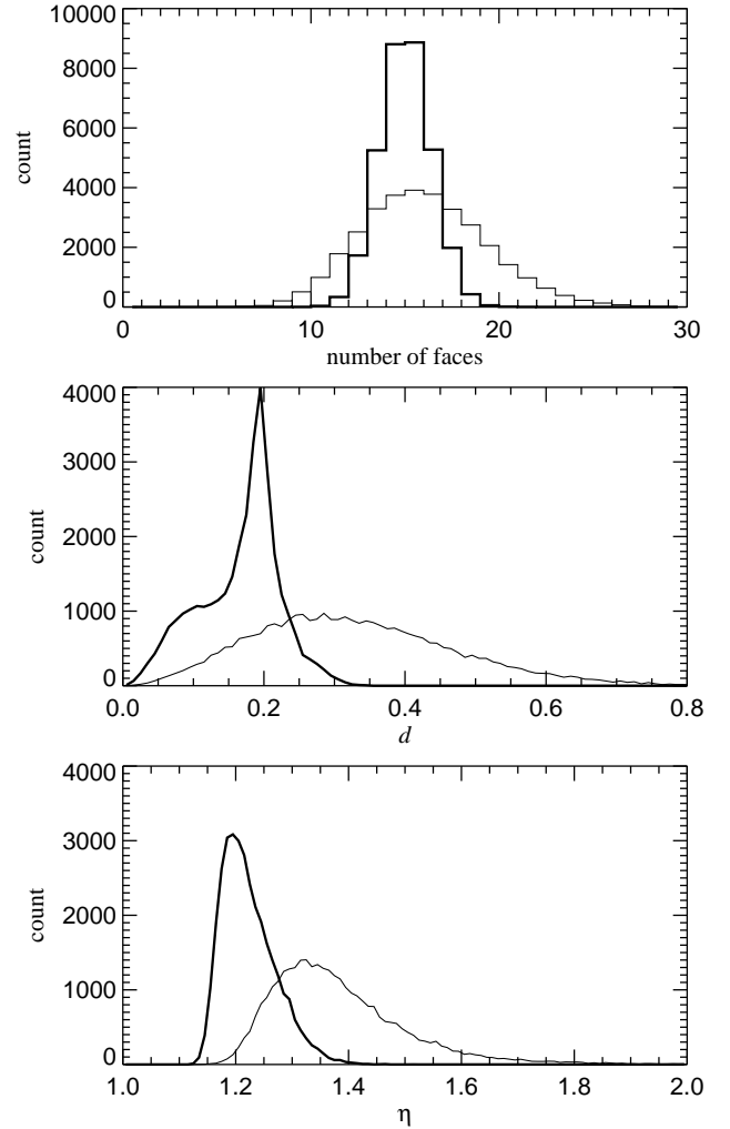
Figure 47. Geometry statistics of the final mesh at z = 0 in our moving-mesh calculation of the Santa Barbara cluster. The histogram in the top panel (thick line) counts the number of faces per cell; the average number is 14.6. The thin line is the same statistic for a Poisson sample ( \sim 15.5 faces per cell on average). The middle panel gives the distribution function of the distance d of mesh-generating points to their cell’s centre-of-masses, in units of the cell radius. Again, we compare the cosmological simulation (thick line) to a Poisson sample (thin line). Finally, the bottom panel gives the distribution of the ratio \eta = S^{3/2} / (6\sqrt{\pi} V) of the surface areas of cells to their volumes.
