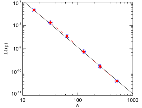
Figure 19. L1 error norm for an acoustic wave in one dimension, calculated with the moving-mesh code (red circles), or with a fixed mesh (blue open circles). The two schemes produce nearly identical errors (the moving mesh code lies only \sim 1-2\% lower), and the solution converges as L1 \propto N^{-2} , i.e. with second order accuracy.
