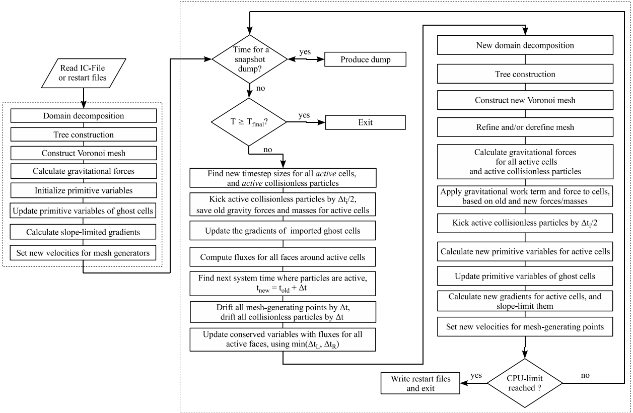
Figure 18. Flow chart of the simulation code. After a number of initialization steps (marked by the dashed box on the left), the code enters a main loop. In each iteration of the main loop, the system advances by a time interval \Delta t that corresponds to the smallest occupied timebin. Active cells or collisionless particles are always those with a timestep that is in sync with the current time of the system. In the first phase, operations correspond to active particles beginning their timestep, in the second phase to those that end their timestep.
