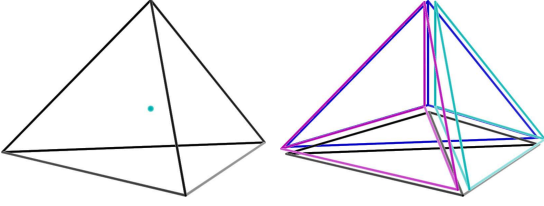
Figure 3. A ‘1-to-4’ flip. A newly inserted point splits its insertion tetrahedron into 4 daughter tetrahedra.
