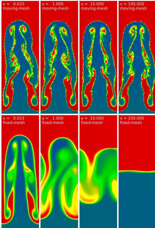
Figure 36. Rayleigh-Taylor instability calculated with different Galilean boosts v_x in the horizontal direction (the simulation domain is periodic in the x direction). The correct result in principal be independent of v . The top row shows the result at time t = 15.0 computed with our moving-mesh approach, while the bottom row of panels gives the corresponding results for a fixed-mesh calculation with AREPO.
