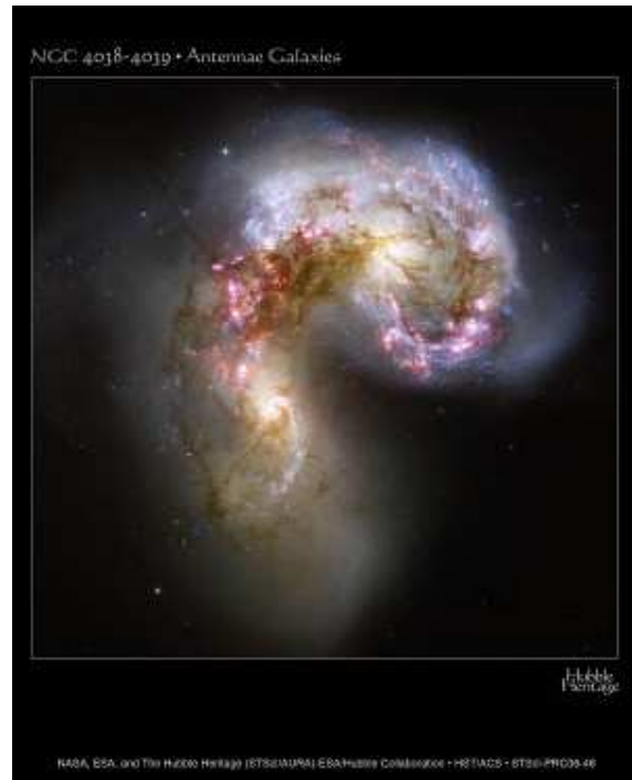
Figure 2.22: This image of the Antennae galaxies shows a multitude of bright young star clusters, groups of stars associated with regions of intense star formation. Credit: NASA, ESA, and the Hubble Heritage (STScI/NASA/ESA/Hubble Collaboration) - HST/ACS - STScI/PHO38-46
