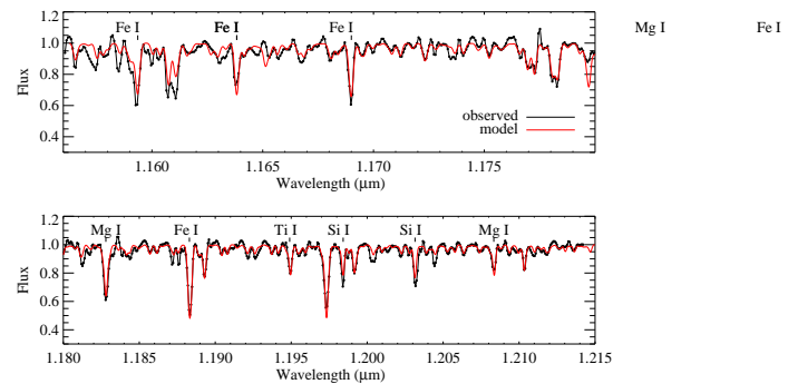
Figure 2.31: Comparison of the observed (black) and theoretical NLTE (red) spectra for Betelgeuse.
