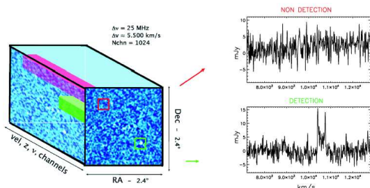
Figure 2.7: A schematic representation of an ALFALFA 3-dimensional data-cube. Each pixel represents a position on the sky (defined by RA and Dec) and a velocity, where each data cube is 2.4 by 2.4 degrees in size and about 5500 km/s in velocity range (25 MHz in frequency). For each pixel a value of the flux density is recorded. For each target, we extract a spectrum over the velocity range from the data-cube at a given position of the sky. Two examples of extracted spectra are shown on the right, illustrating an HI detection (bottom) and an HI non-detection (top). Image credit: Fabello, S. et al, 2011, MNRAS, 411, 993.
