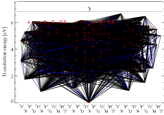
Figure 2.29: Complete atomic model for the neutral Ti.
