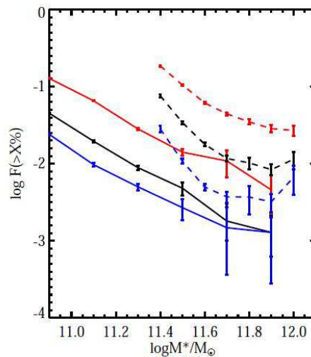
Figure 2.3: The solid red, black and blue lines show the fraction of galaxies that have formed more than 5, 10 and 15% of their stars in the last billion years as a function of stellar mass. These results are for galaxies with median redshift z=0.1 in the SDSS low redshift main sample. The dashed red, black and blue lines show the same thing for galaxies with median redshift z=0.5 in the BOSS sample.
