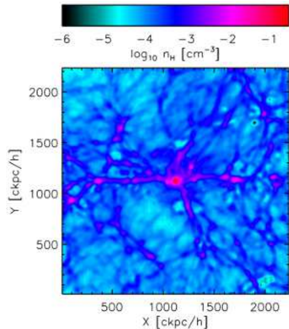
Figure 2.17: Example of the inhomogeneous intergalactic medium around a Lyman-alpha emitter. The colouring indicates the number density of hydrogen atoms with the scale given at the top.
